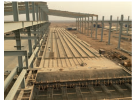
El Seif Precast have increased their existing 8 beds with another 16 beds at the city of Jizan
